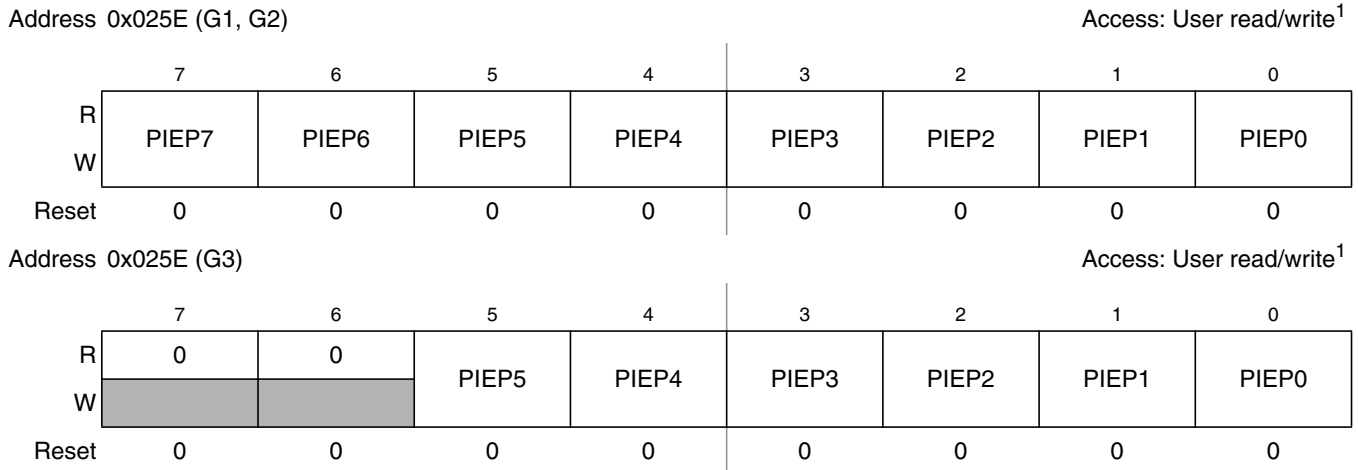
Figure 2-40. Port P Interrupt Enable Register (PIEP)
