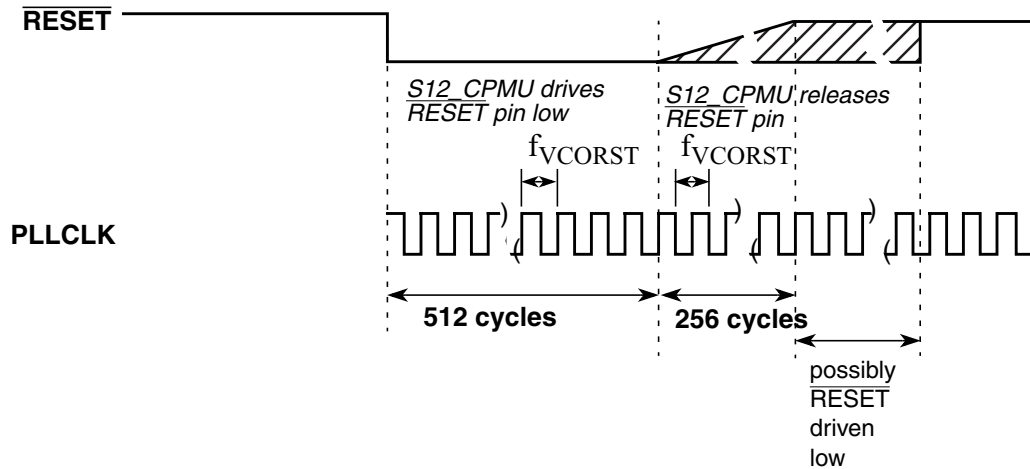
Figure 10-34. RESET Timing
