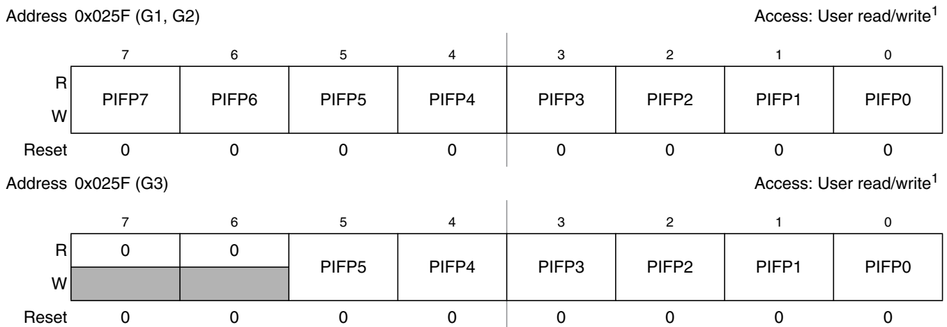
Figure 2-41. Port P Interrupt Flag Register (PIFP)
